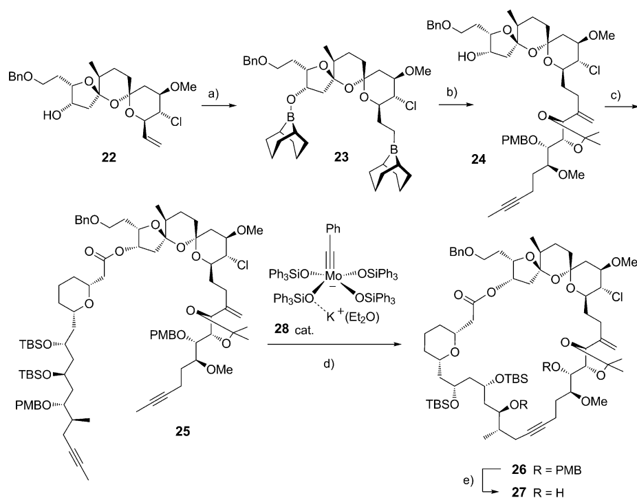
Scheme 4. a) 9-H-9-BBN dimer, THF; b) aq NaOH (1 M), [PdCl 2 (dppf)] (20 mol %), Ph 3 As (20 mol %), 21 , THF, 76%; c) 1. 9 , 2,4,6-trichlorobenzoyl chloride, Et 3 N, toluene, 0°C; 2. 24 , DMAP, toluene, 0°C→RT, 85%; d) 28 (8 mol %), 5 Å M.S., toluene, 87%; e) DDQ, CH 2 Cl 2 , 0°C→RT, 91%. 9-BBN = 9-borabicyclo[3.3.1]nonane, dppf = 1,1'-bis(diphenylphosphino)ferrocene, DMAP = 4-dimethylamino-pyridine; M.S. = molecular sieves.
